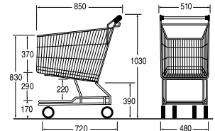
Ref. 7 767 25 03 Nesting distance: 231 mm
