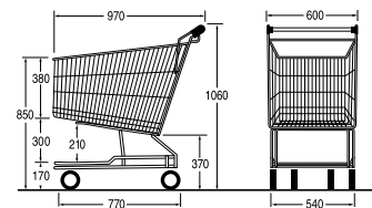
Ref. 7 767 80 03 Nesting distance: 249 mm
