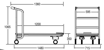
Ref. 4 459 70 03 Nesting distance: 340 mm Permitted load: 350 kg
