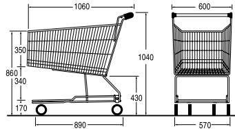
Ref. 7 734 60 03 Nesting distance: 220 mm
