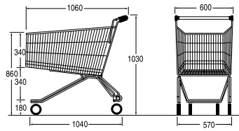
Ref. 7 735 00 03 Nesting distance: 220 mm
