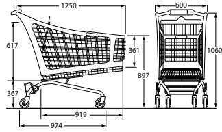
Ref. 7 786 04 03 Nesting distance: 295 mm
