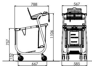
Ref. 7 900 25 03 Nesting distance: 260 mm * No available for moving walkway
