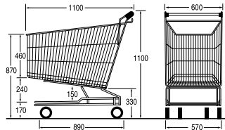
Ref. 7 767 40 03 Nesting distance: 250 mm
