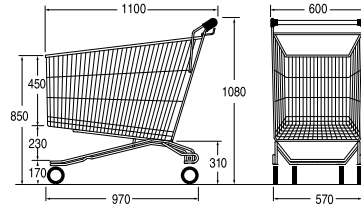
Ref. 7 770 10 03 Nesting distance: 230 mm
