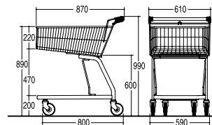
Ref. 7 788 80 03 Nesting distance: 225 mm
