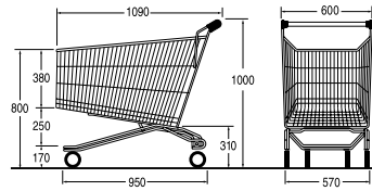
Ref. 7 798 32 03 Nesting distance: 250 mm
