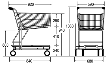
Ref. 4 455 00 03 Nesting distance: 270 mm
