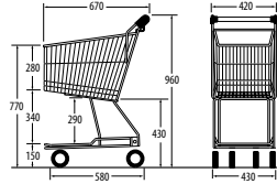
Ref. 7 768 62 03 Nesting distance: 175 mm
