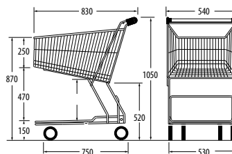
Ref.7 729 00 03 Nesting distance: 145 mm
