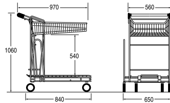
Ref. 4 455 03 03 Nesting distance: 270 mm
