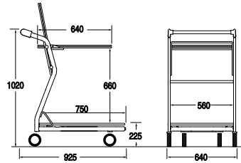
Ref. 4 454 08 03 Nesting : 242 mm
