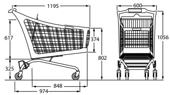
Ref. 7 786 02 03 Nesting distance: 285 mm
