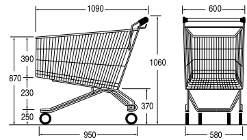
Ref. 7 722 90 03 Nesting distance: 230 mm
