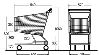
Ref. 7 767 50 03 Nesting distance: 259 mm
