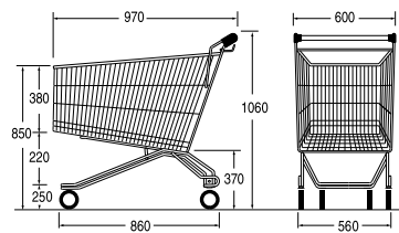
Ref. 7 722 80 03 Nesting distance: 230 mm
