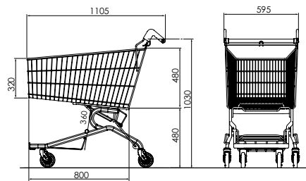
Ref. 7 780 03 03 Nesting distance: 270 mm
