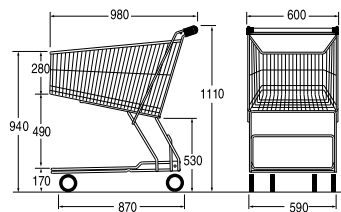
Ref.7 727 50 03 Nesting distance: 210 mm
