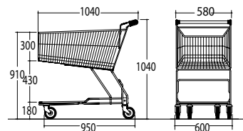
Ref. 7 795 30 03 Nesting distance: 235 mm
