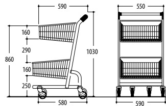
Ref. 7 788 12 03 Nesting : 190 mm 10 nested trolleys: 1769 mm Product with options
