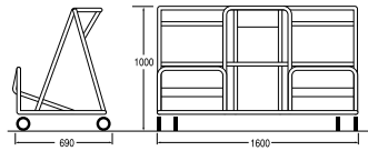
Ref. 4 436 30 38 Nesting distance: 255 mm Permitted load: 300 kg
