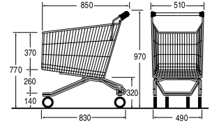
Ref. 7 778 32 03 Nesting distance: 215 mm
