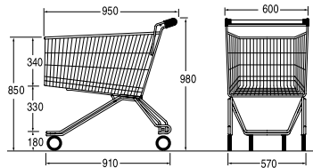
Ref. 7 721 20 03 Nesting distance: 220 mm
