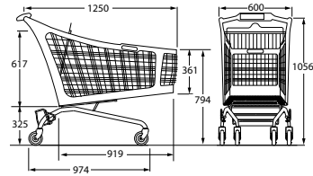
Ref. 7 786 01 03 Nesting distance: 285 mm
