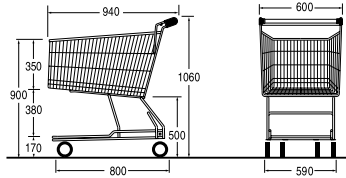
Ref. 7 795 00 03 Nesting distance: 266 mm
