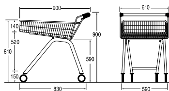
Ref. 7 788 70 03 Nesting distance: 250 mm
