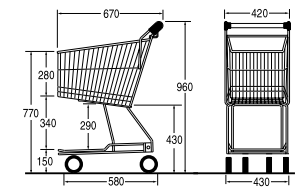
Ref. 7 768 62 03 Nesting distance: 175 mm
