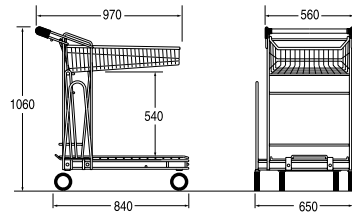
Ref. 4 455 90 03 Nesting distance: 270 mm
