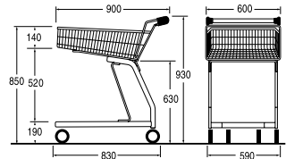
Ref. 7 788 51 03 Nesting distance: 250 mm
