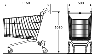
Ref. 7 780 01 03 Nesting distance: 240 mm
