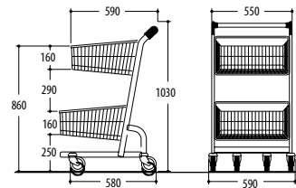
Ref. 7 788 12 03 Nesting distance: 190 mm
