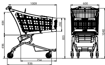
Ref. 7 786 03 03 Nesting distance: 270 mm
