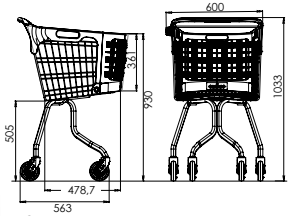
Ref. 7 784 01 03 Nesting distance: 150 mm Registered design
