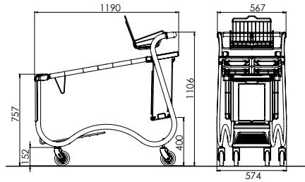
Ref. 7 900 15 03 Nesting distance: 260 mm * No available for moving walkway
