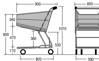
Ref.7 727 25 03 Nesting distance: 190 mm
